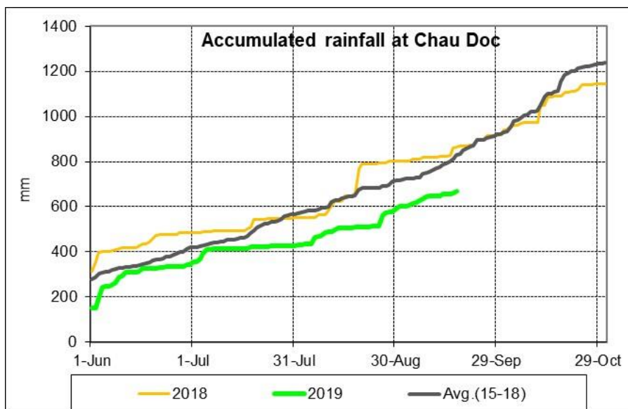
Figure 4: Accumulated Rainfall up to 17 th September to 2019 in specific stations over the LMB
