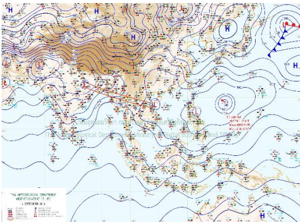
Figure 1: Weather map for 12 th Sept 2019
