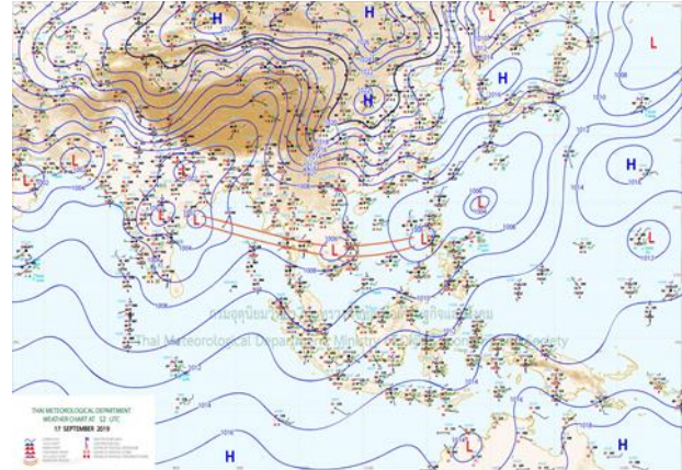
Figure 2: Weather map for 17 th Sept 2019
