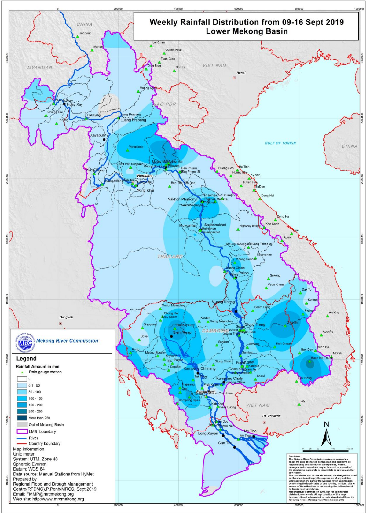
Figure 3: Weekly Rainfall Distribution over the LMB from 09 th to 16 th Sept 2019
